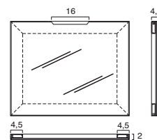
door deep drawer with aluminium frame brill finish, incorporated handle W 160 mm with glossy amber (code 723A)
